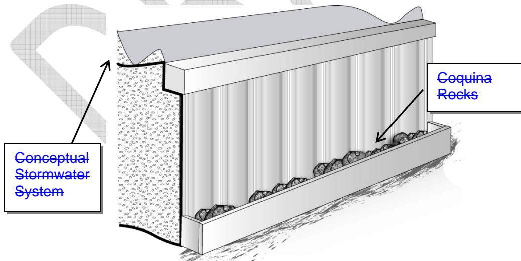
Sheet bulkhead without pilings and swale drainage.
