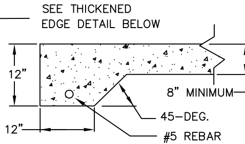
THICKENED EDGE DETAIL
