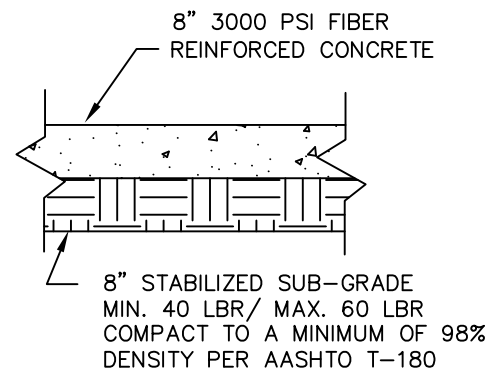
CONCRETE APRON DETAIL
